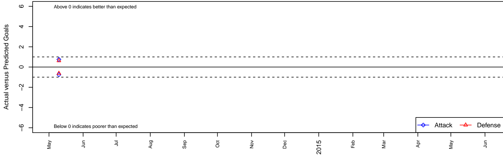
Flathead Force Green G99 Dots are actual minus expected GF (blue circles) and GA (red triangles). Blue line is smoothed change in attack strength. Red is smoothed change in defense strength.
